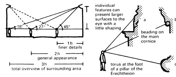
⑧ Street widths play an important role in the level of detail which is perceived from ground level ⑨ Parts of buildings meant to be seen but sited above projections must be placed sufficiently high up (see a)
